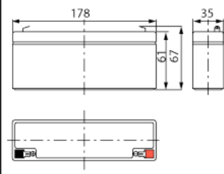
Dimensions (mm)
